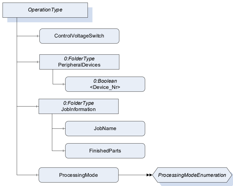
Figure 15 – Overview of OperationType
