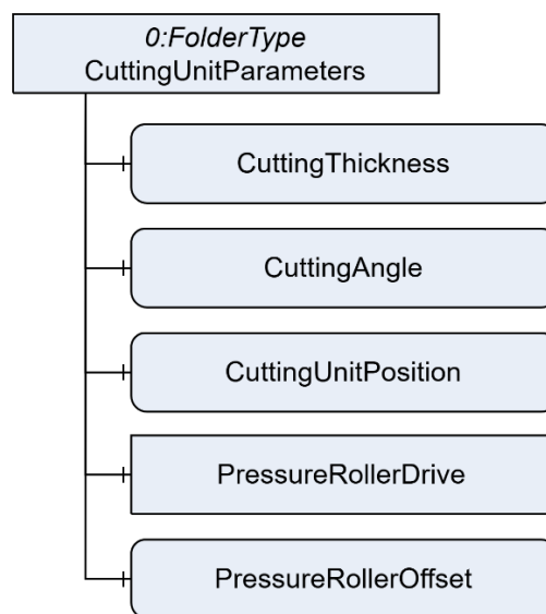
Figure 9 – Cutting Unit Parameters Overview
