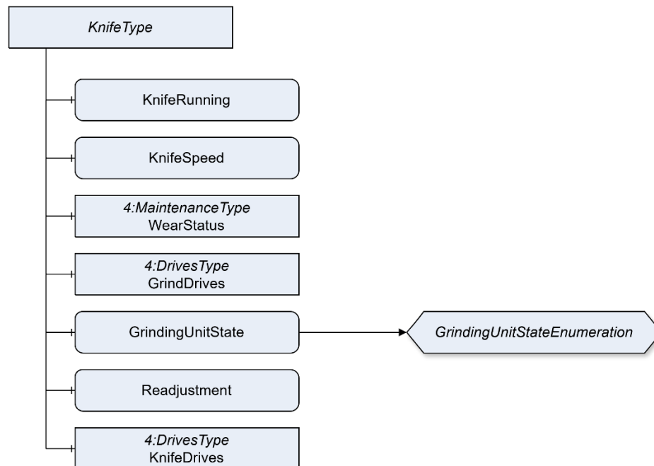
Figure 13 – KnifeType overview
