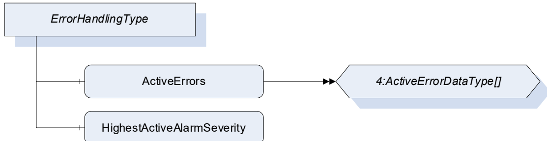
Figure 16 – Overview of ErrorHandlingType
