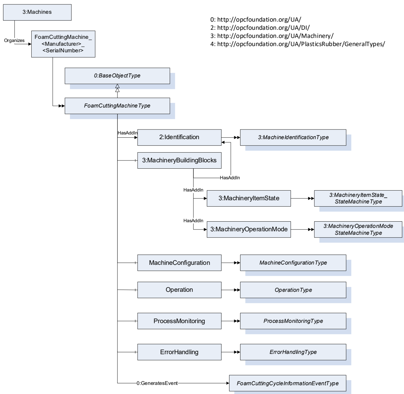
Figure 1 – FoamCuttingMachineType Overview
