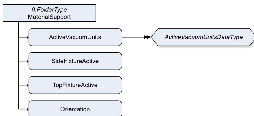
Figure 10 – Material Support Overview
