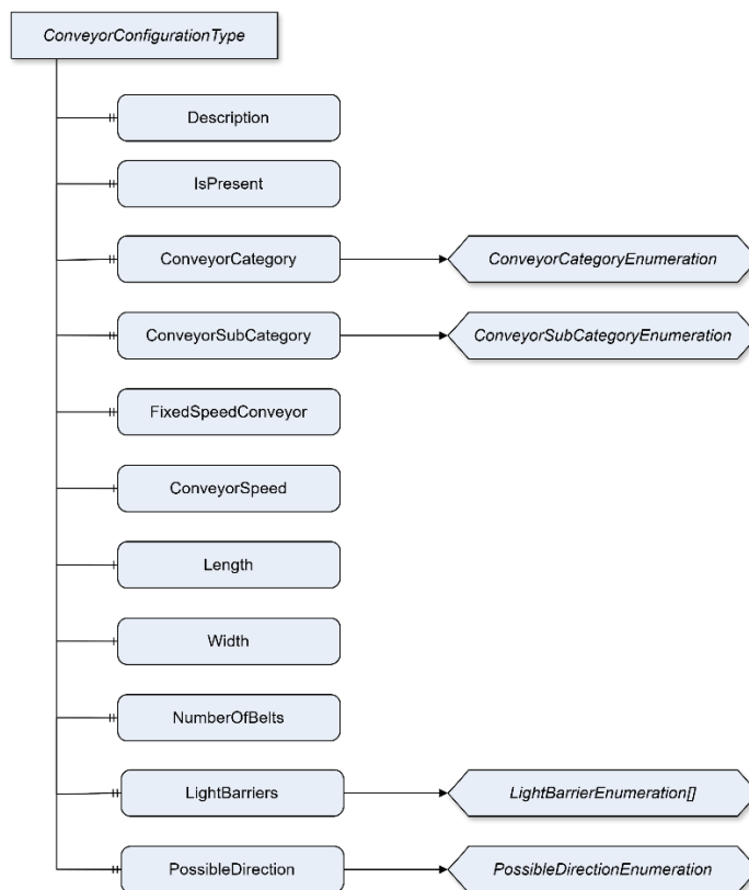
Figure 3 – ConveyorConfigurationType Overview
